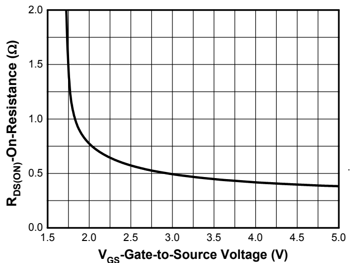
On Resistance vs. V_{GS}
