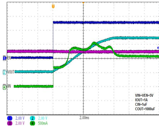
Startup from Enable ON (WS4611A)
