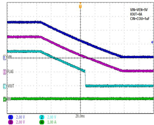
Shutdown from Power OFF (WS4611A)
