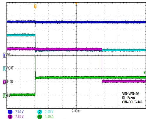
Current Limit Response (WS4611A)
