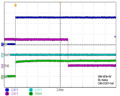
Start into Short Circuit (WS4611A)
