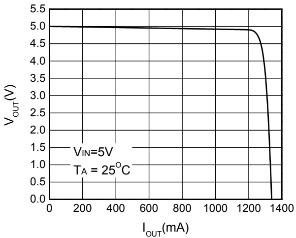
Output Voltage vs. Output Current (WS4611A)
