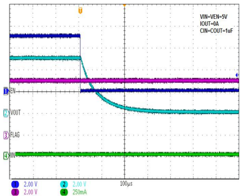
Shutdown from Enable OFF (WS4611A)
